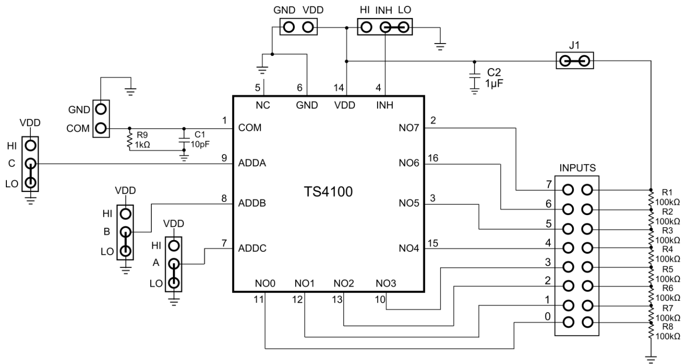
Figure 3. TS4100 Demo Board Circuit
