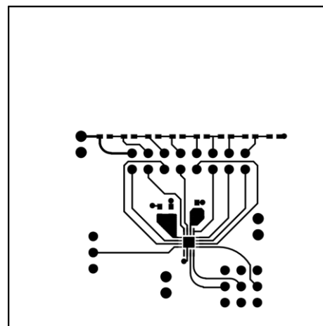
Figure 5. Top Layer View #2
