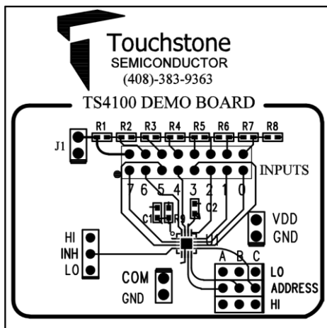
Figure 4. Top Layer View #1
